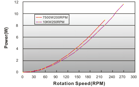
GL-PMG-7500 PMG Power Curve
