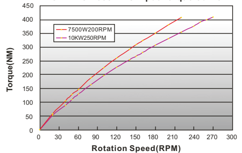
GL-PMG-7500 PMG Input Torque Curve
