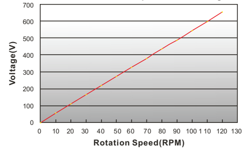
GL-PMG-20K PMG Open Circuit Voltage
