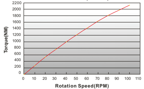
GL-PMG-20K PMG Input Torque Curve
