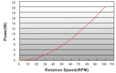
GL-PMG-20K PMG Power Curve
