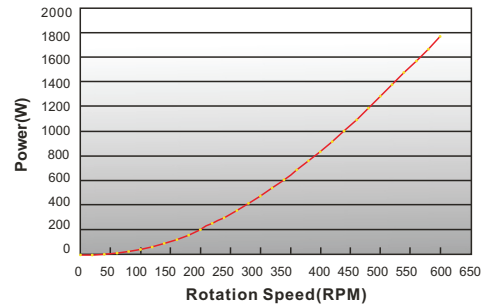
GL-PMG-1500 PMG Power Curve
