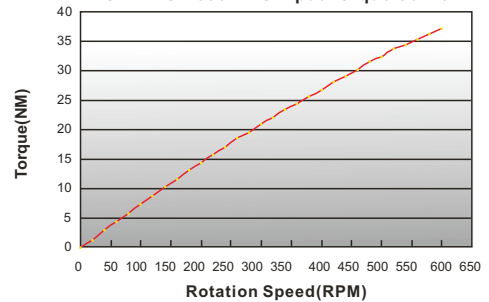
GL-PMG-1500 PMG Input Torque Curve
