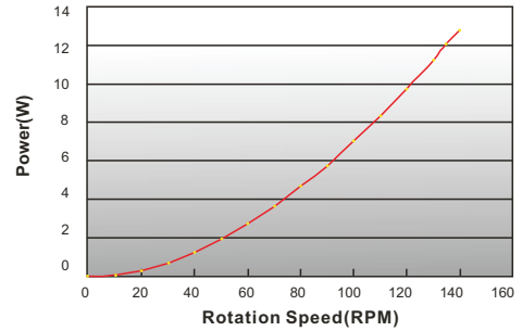
GL-PMG-12K PMG Power Curve
