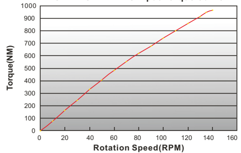
GL-PMG-12K PMG Input Torque Curve
